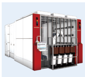
Horizontal furnaces
